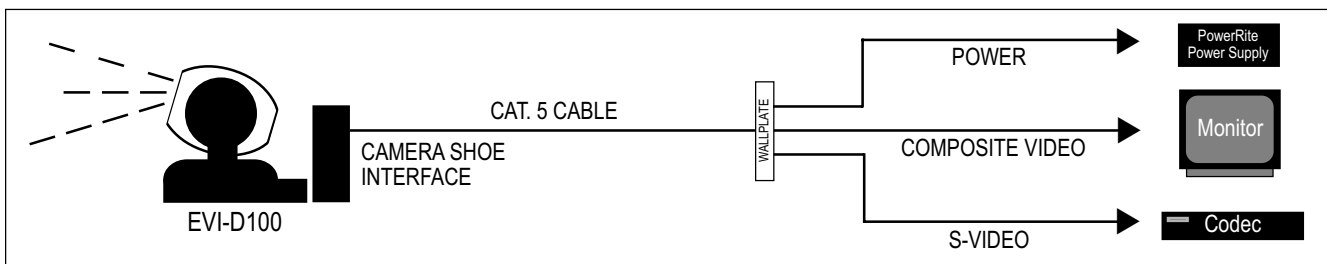
Figure 1 – EZCamera cable system with a quick-connect single gang wallplate/quick-connect box.
