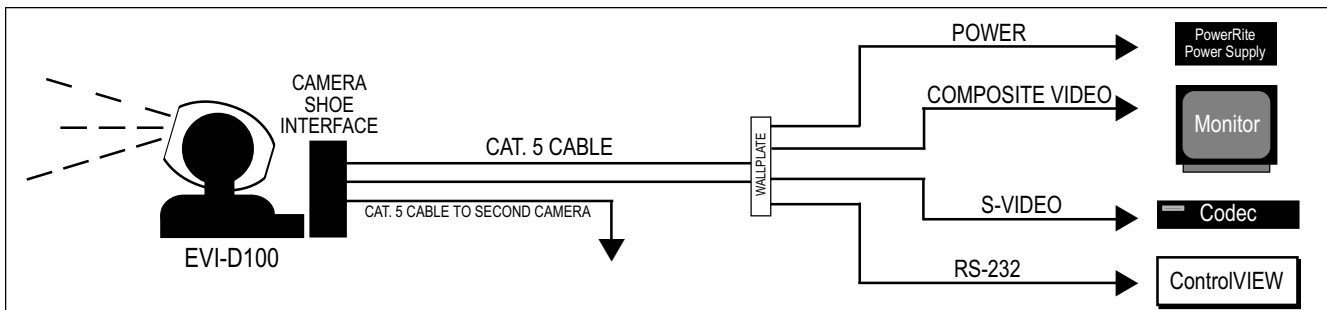
Figure 2 – EZCamera cable system with a quick-connect dual gang wallplate.
